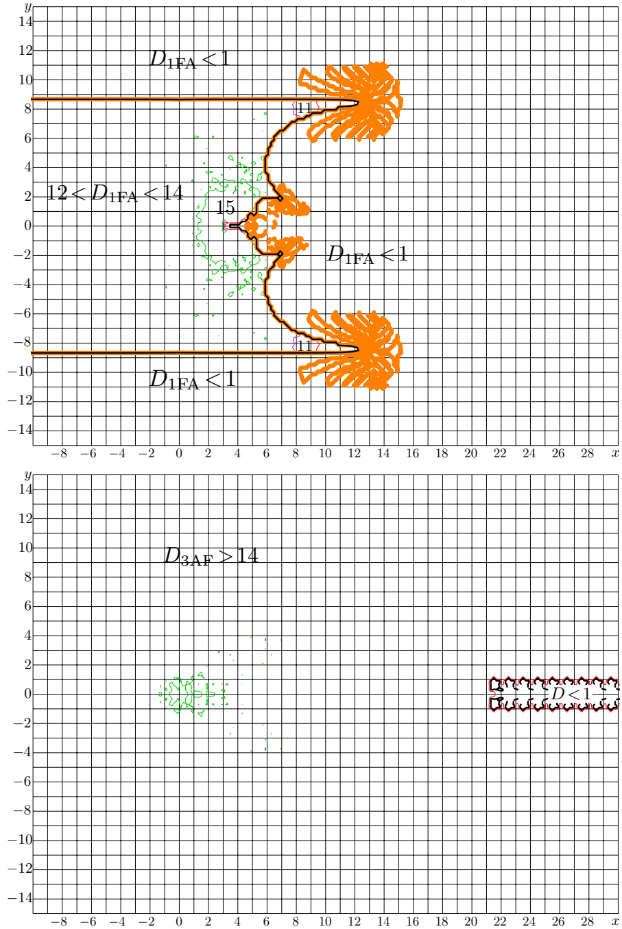
FIGURE 4. The agreements D = D_{1FA}(z) and D = D_{3AF}(z) and in the complex plane z = x+iy ; level D=1 is shown with thick lines; the integer values are shown with thin lines; levels D=2 is shown with black thick lines, levels D = 1, 2, 10, 12, 14 are seen; symbols “15” and “11” indicate the ranges where D > 14 and 10 > D > 12 .
